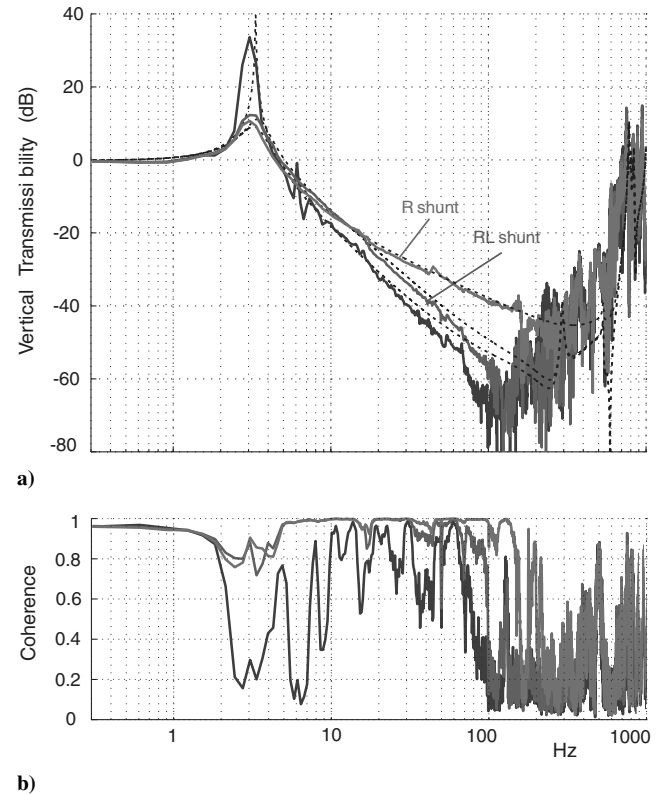
Fig. 17 Experimental results of vertical transmissibility and coherence function (zero-gravity parabolic flight). The numerical predictions are in dotted lines.
