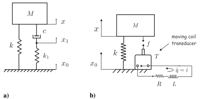
Fig. 4 Illustrations of the a) relaxation isolator consisting of a spring in parallel with a Maxwell unit and b) electromagnetic realization with a voice coil and a R - L circuit.
