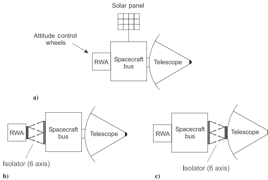
Fig. 2 Spacecraft architecture: a) without isolator, b) isolator placed between the RWA and the spacecraft bus, and c) isolator between the spacecraft bus and the telescope.
