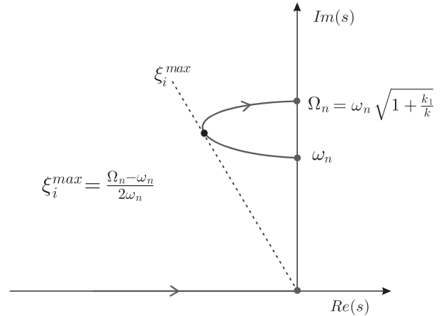
Fig. 6 Root locus of the solutions of Eq. (6) as c goes from zero to infinity. The maximum damping is achieved for k_1/c = \Omega_n^{3/2}/\omega_n^{1/2} .
