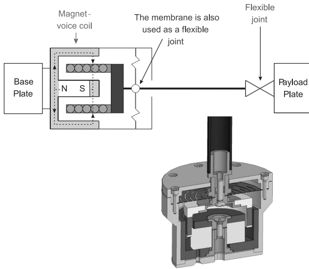
Fig. 11 The leg of the passive isolator.
