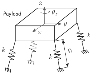
Fig. 8 Six-axis isolator.
