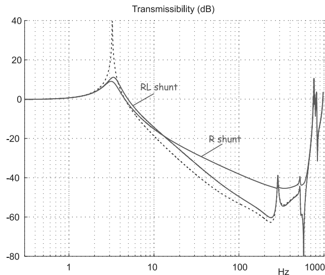
Fig. 14 Numerical comparison of the vertical transmissibility: open-loop (dotted line), relaxation isolator (RL shunt), and linear viscous (R shunt).
