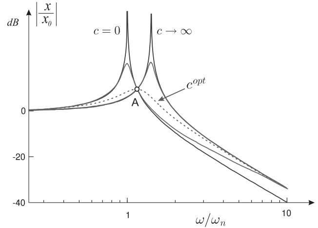
Fig. 5 Transmissibility of the relaxation oscillator for fixed values of k and k_1 and various values of c . The first peak corresponds to \omega = \omega_n ; the second one corresponds to \omega = \Omega_n . All the curves cross each other at A and have an asymptotic decay rate of -40 dB/decade. The curve corresponding to c_{opt} is nearly maximum at A.
