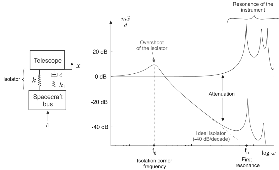
Fig. 1 Effect of the isolator on the transmissibility between the spacecraft bus and the telescope.
