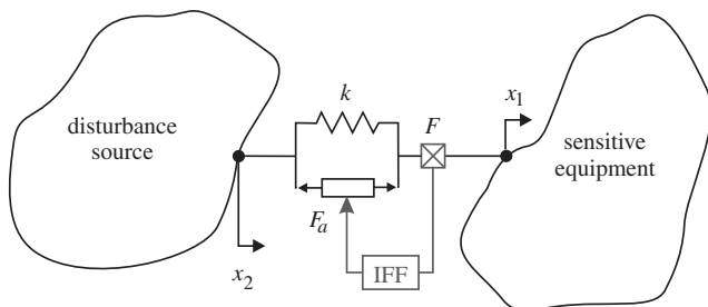
Fig. 3 Two arbitrary flexible structures connected by a single-axis soft isolator with force feedback. The open-loop transfer function F/F_a exhibits alternating poles and zeros.
