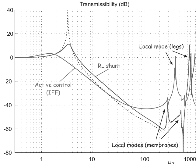
Fig. 13 Numerical comparison of the vertical transmissibility: open-loop (dotted line), relaxation isolator (RL shunt), and skyhook (IFF).
