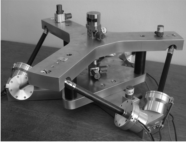
Fig. 10 View of the isolator.
