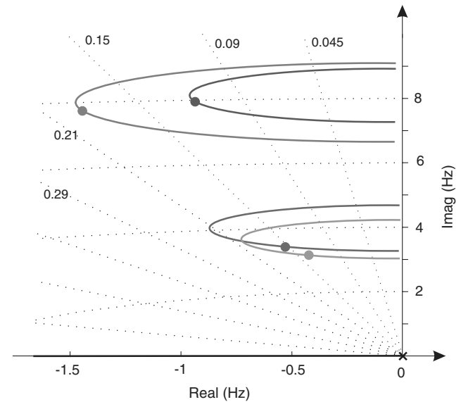
Fig. 9 Root locus of the six-axis relaxation isolator (there are only four different curves because of the symmetry of the system). The bullets correspond to the design values.
