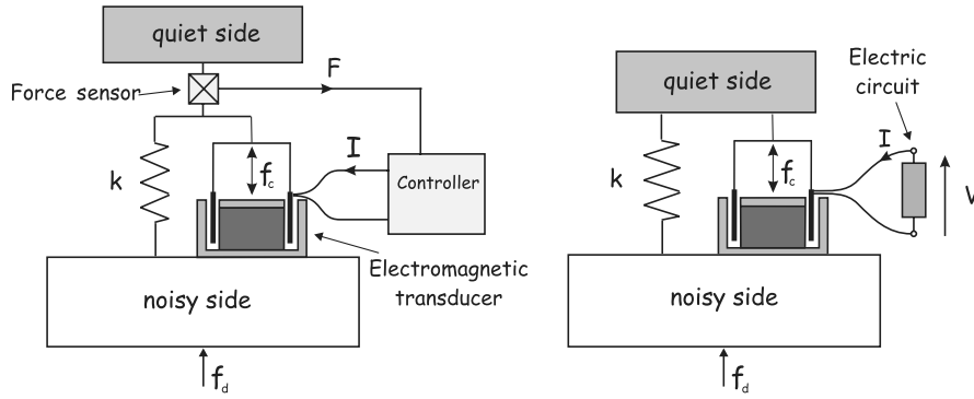
Fig. 7 Comparison of the active isolator (left) with the passive isolator (right); if a RL electrical circuit is used, the passive isolator is a relaxation isolator; a purely resistive circuit produces a linear viscous isolator.
