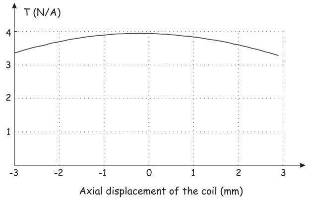
Fig. 12 Evolution of the transducer constant T with the axial displacement of the coil (FE simulations).
