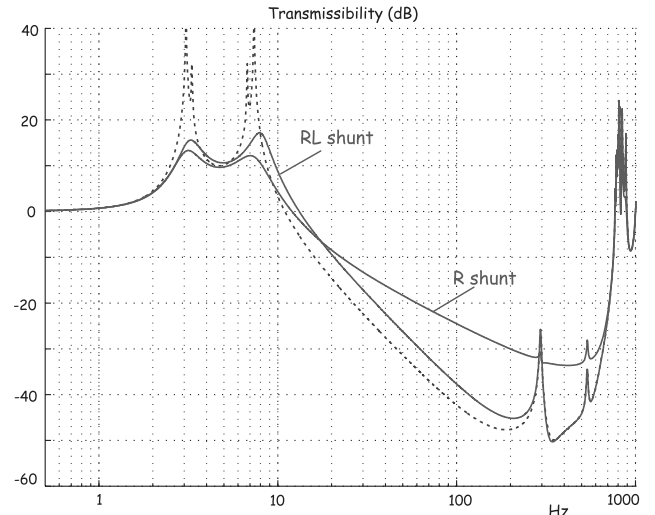
Fig. 16 Numerical comparison of the transmissibility (Frobenius norm of the transmissibility matrix): open-loop (dotted line), relaxation isolator (RL shunt), and linear viscous (R shunt).
